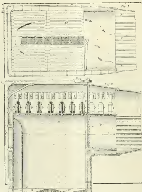
HEAD'S FIRE BOX. FIG. 65.
